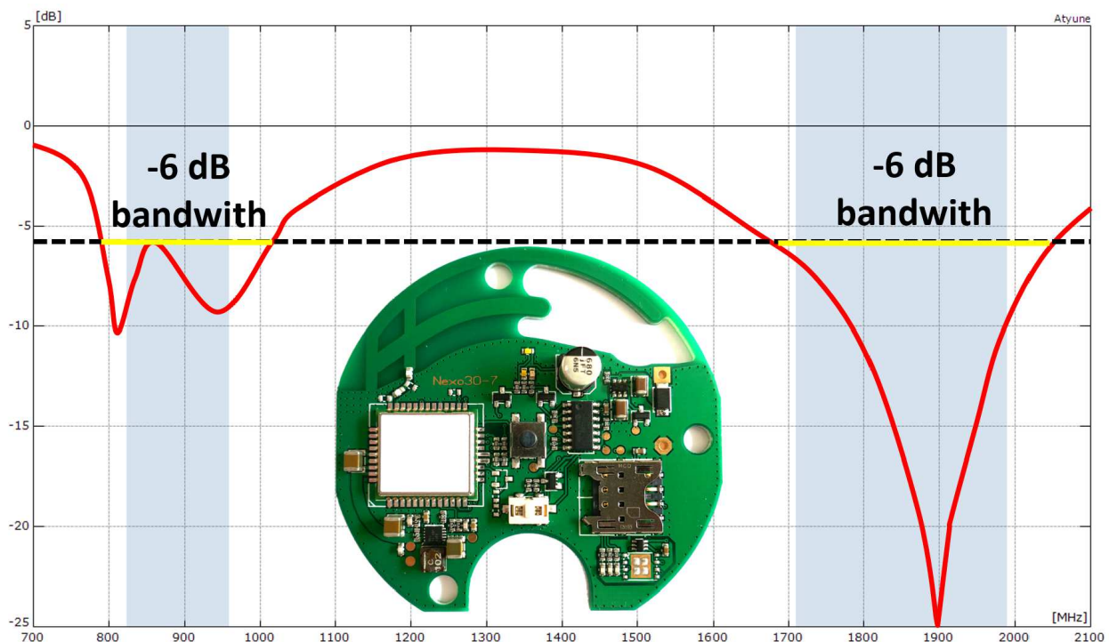
4 Bandwidth with -6 dB return loss of the GSM / NB-IoT / LTE-M PCB antenna at Gillette order button. Source: IoT / M2M Cookbook.
