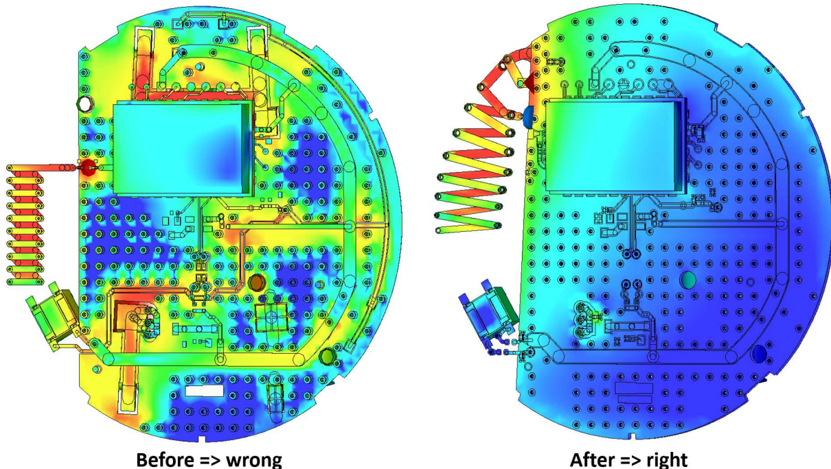
84 Before and after with a LoRaWAN sensor
