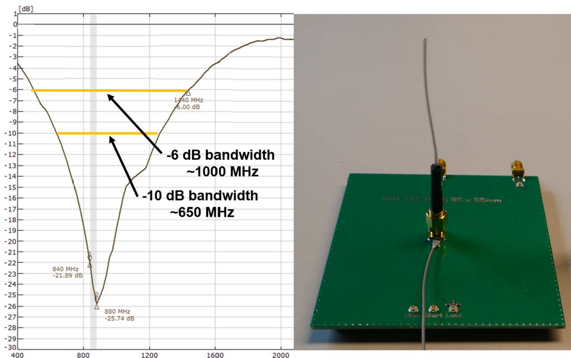
8 Testing of DIY wire antenna on test PCB
