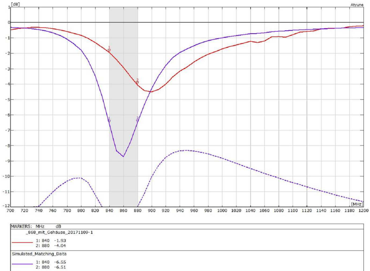
82 LoRa helical antenna matched
