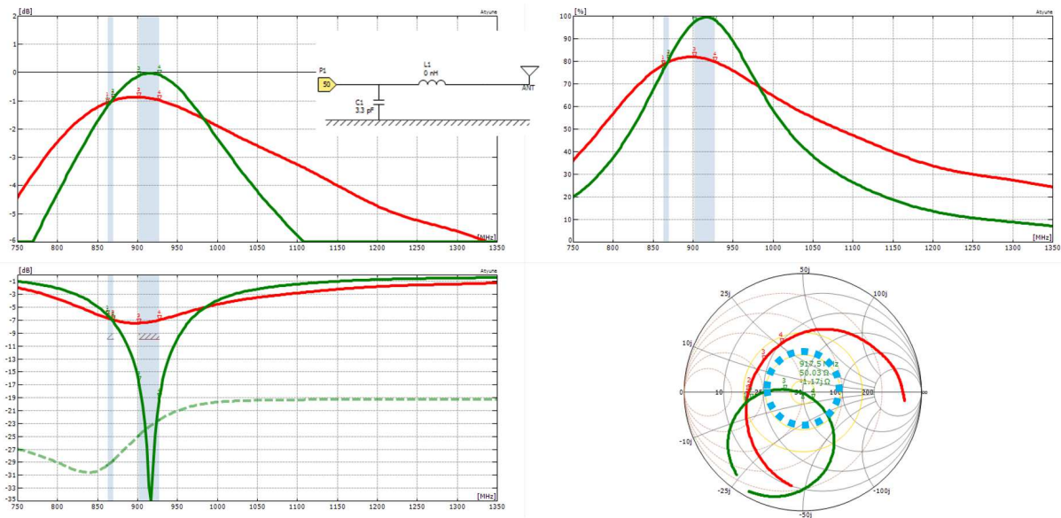
17 Gain, efficiency, return loss and Smith Chart of the L-antenna with change of distance of radiator to ground plane, unmatched and matched version 1 (A1)
