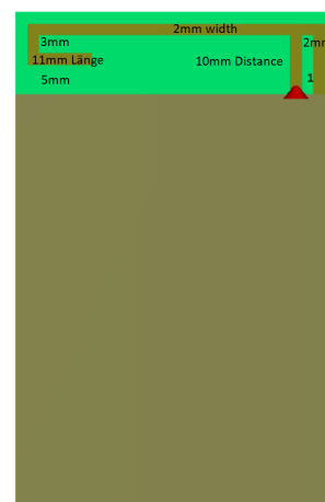
26 F antenna general distances and dimensions
