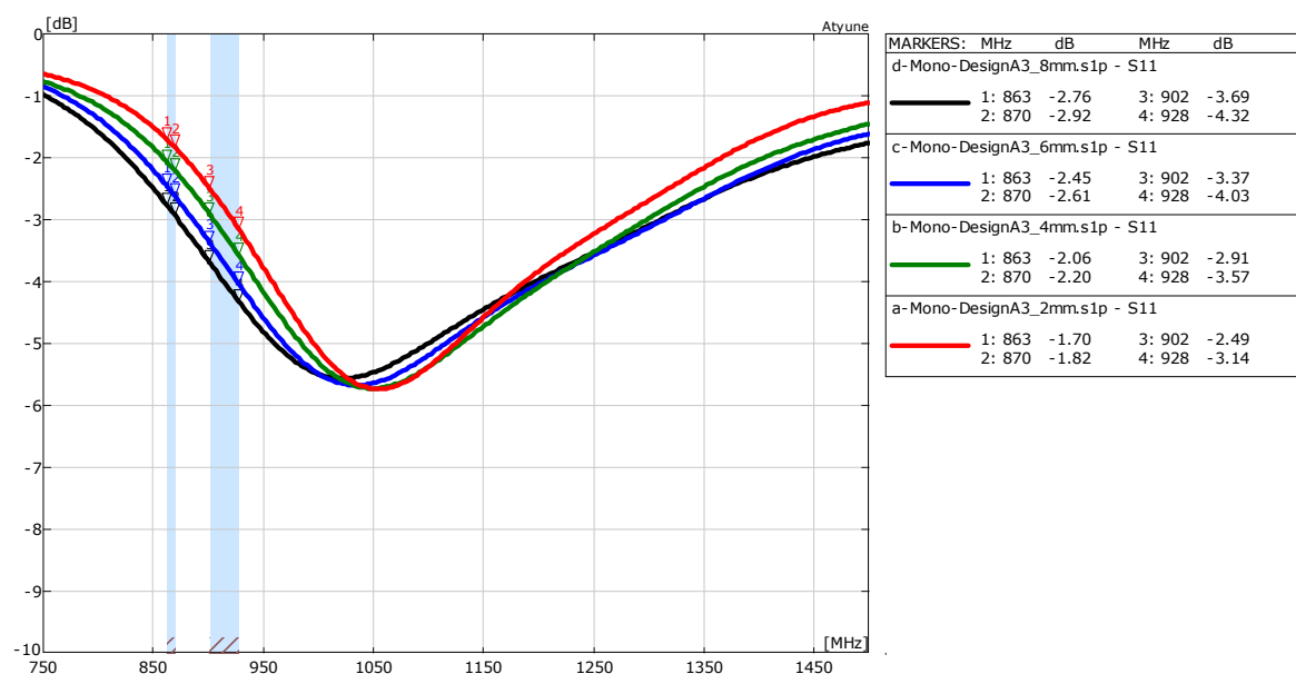
25 Return loss of L-antenna with change of radiator track width
