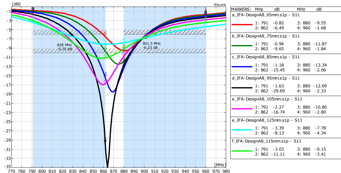
49 Return loss of F antenna with change in length of PCB (A8)
