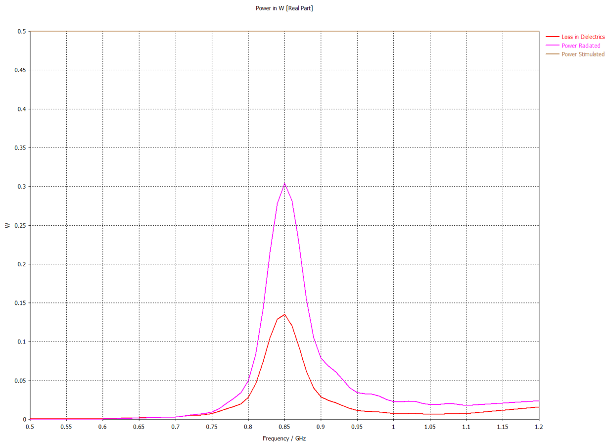
77 Loss in dielectrics, power radiated, power stimulated at 850 MHz centre frequency
