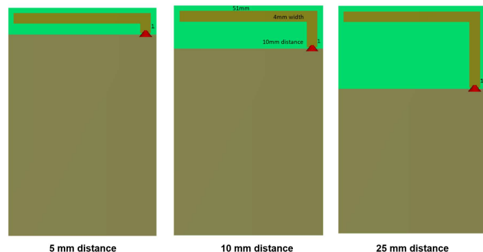
10 L-antenna with change of distance of radiator to ground plane (A1)
