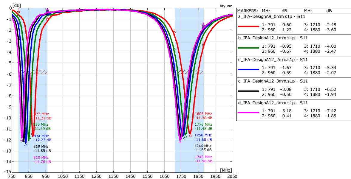
63 Return loss dual F antenna and thickness of the housing (A12)
