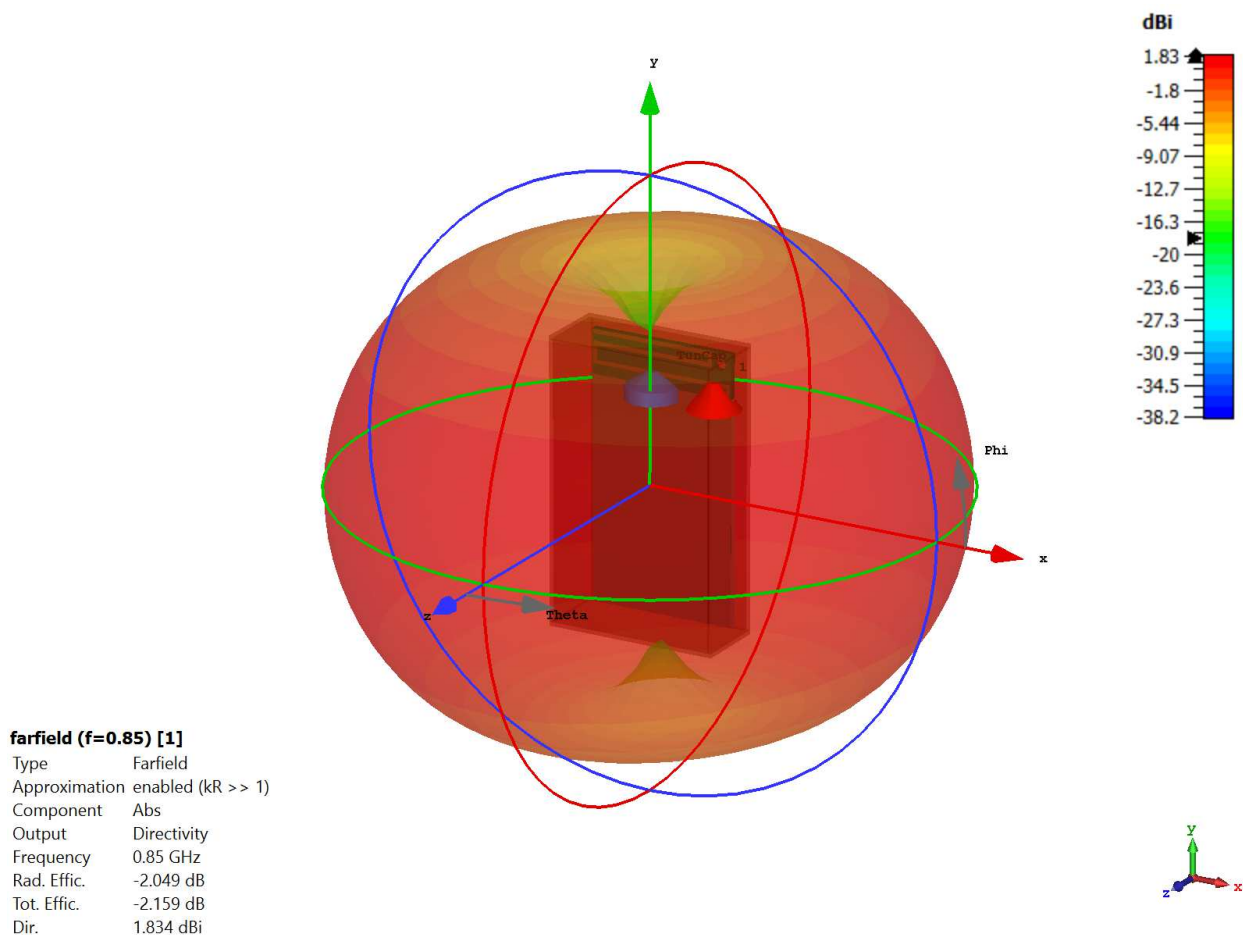
72 Simulation of the radiated energy in 3D at 850 MHz
