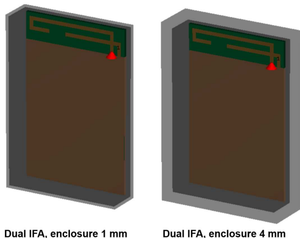
62 Dual F antenna and thickness of the housing (A12)
