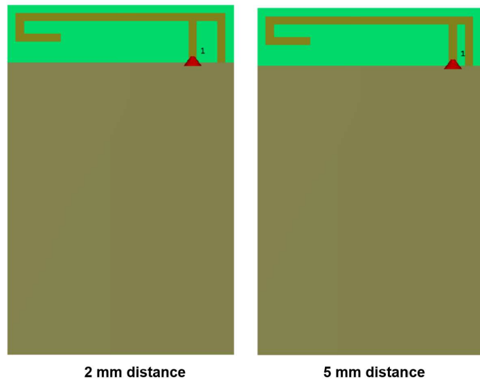
33 F antenna with change of distance to short-circuit point (A4withA8)
