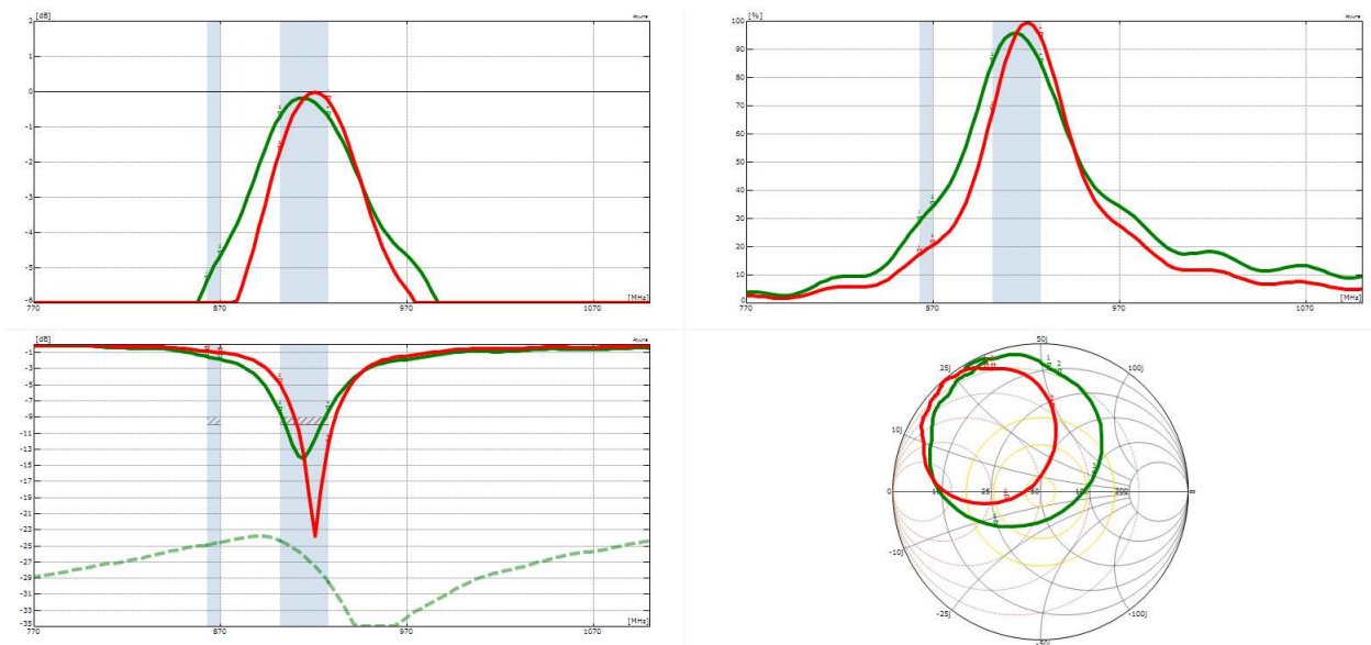
69Gain, efficiency, return loss and Smith Chart for antenna IV
