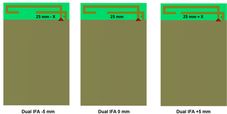
58 Dual F antenna with change in length of radiator (A9)
