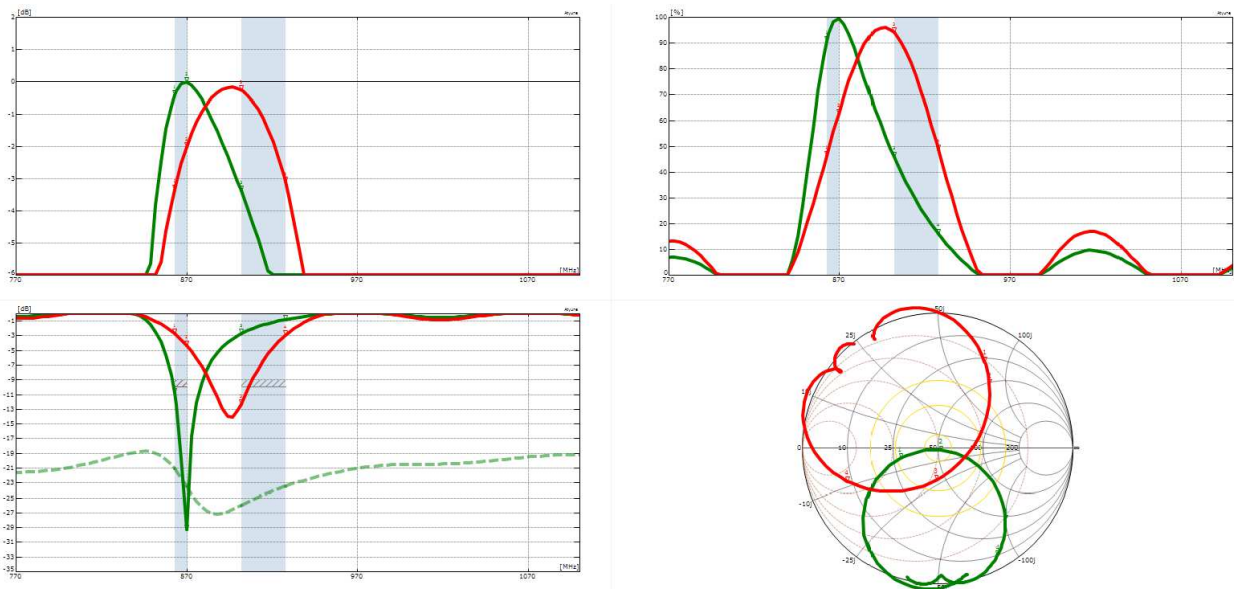
68 Gain, efficiency, return loss and Smith Chart for antenna III
