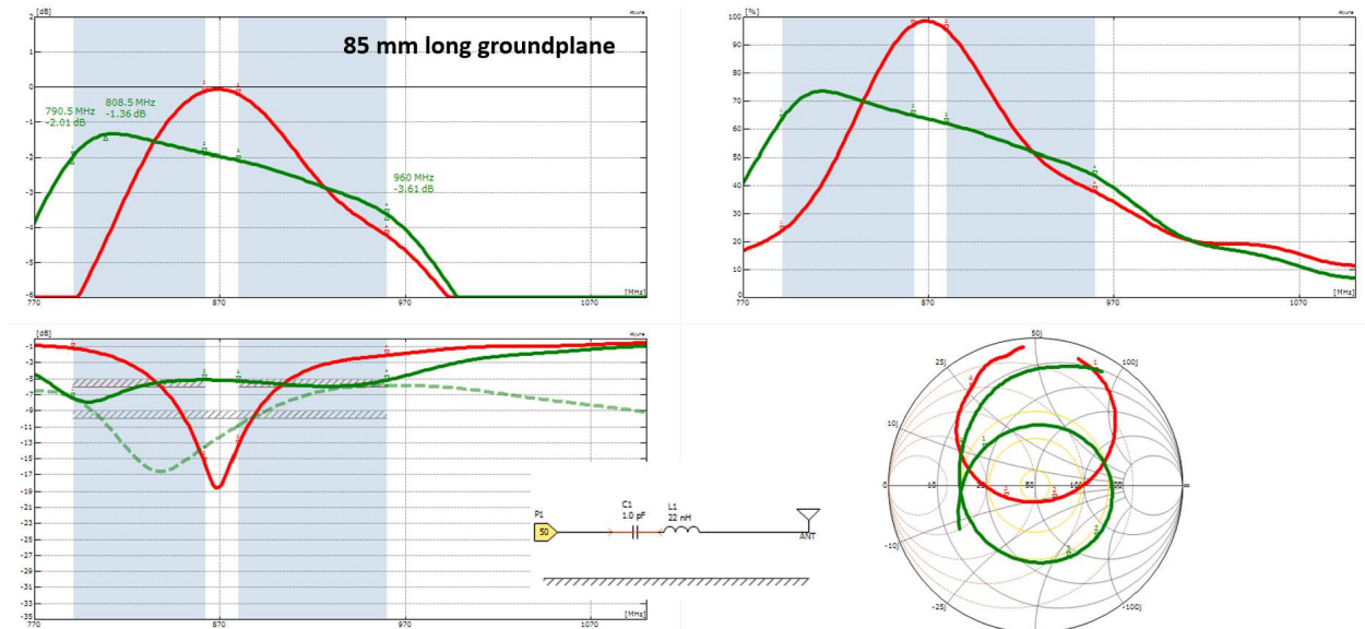
53 Gain, efficiency, return loss and Smith Chart of F antenna a PCB length of 85 mm(A8)
