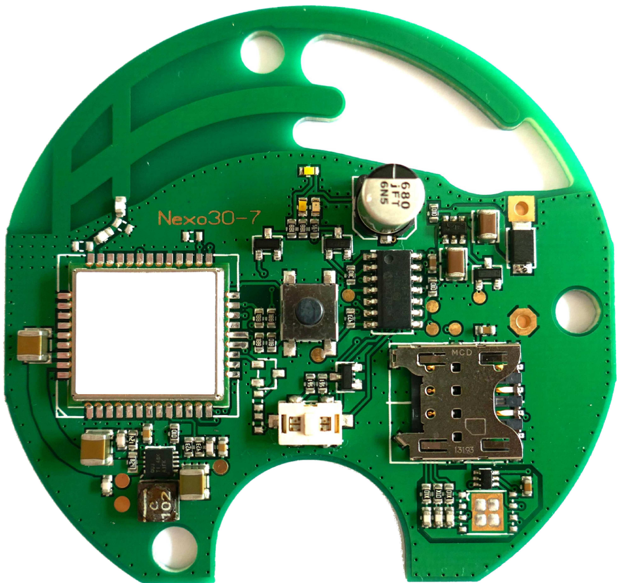
90 Dual F antenna for NB-IoT, LTE-M and GSM at the PCB of the Gillette order button
