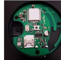
PIFA antenna & three AA cells
