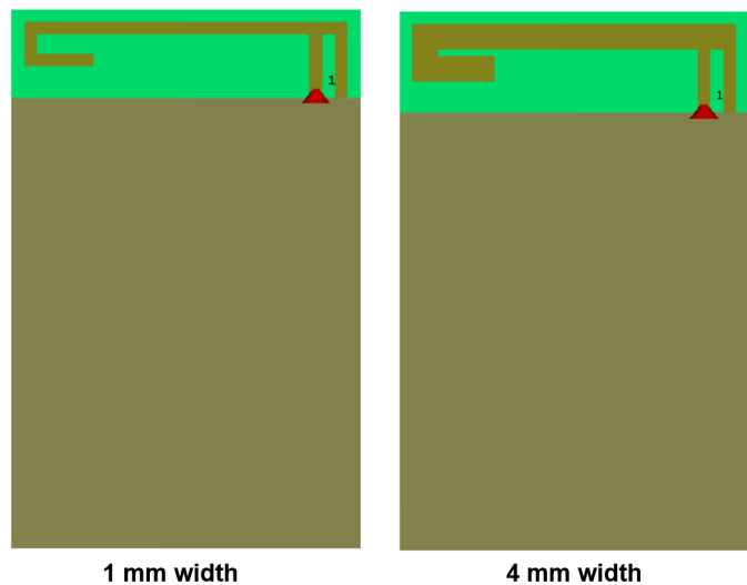
37 F antenna with change of radiator width (A5withA8)
