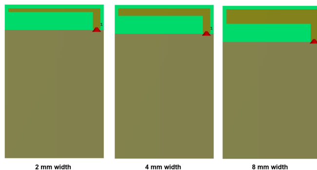
24 L-antenna with change of radiator track width
