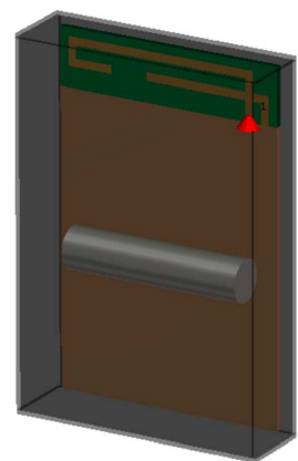
Dual IFA with battery V3
