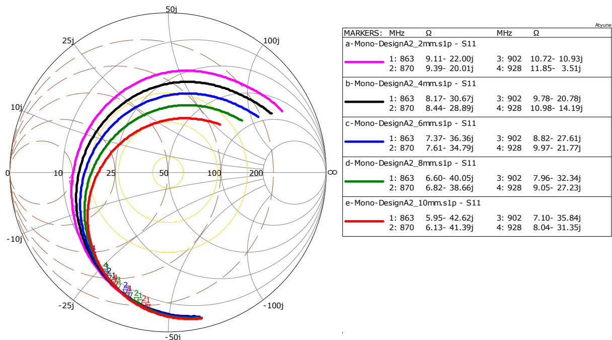
23 Smith chart of the L-antenna with change of trace width at feed point
