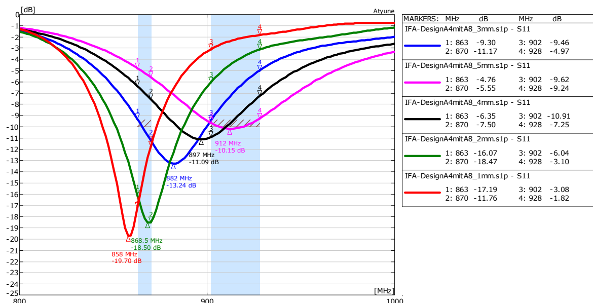
34 Return loss of F-antenna with change of distance to short-circuit point (A4withA8)
