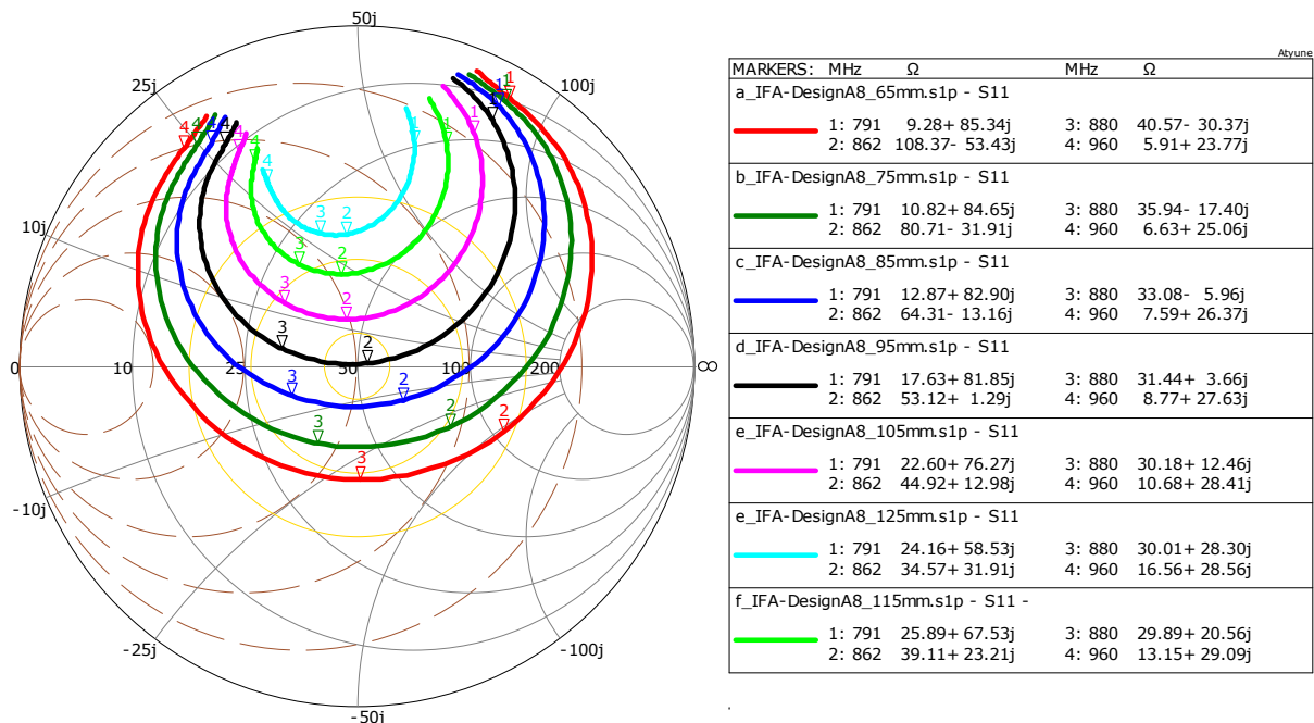
50 Smith chart of F antenna with change in length of PCB (A8)
