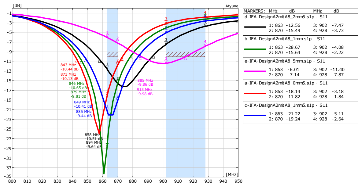
30 Frequency bandwidth at -10 dB return loss for A2withA8
