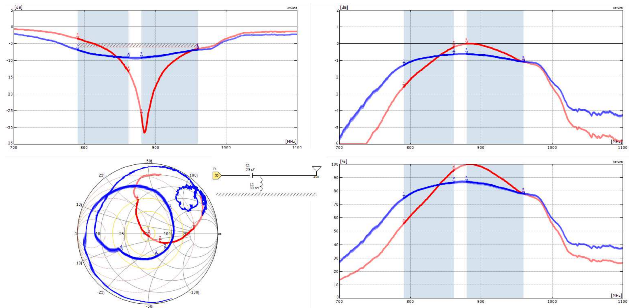
88 Gain, efficiency, return loss and Smith Chart of inverted F antenna for 868 MHz optimised for 791 - 960 MHz
