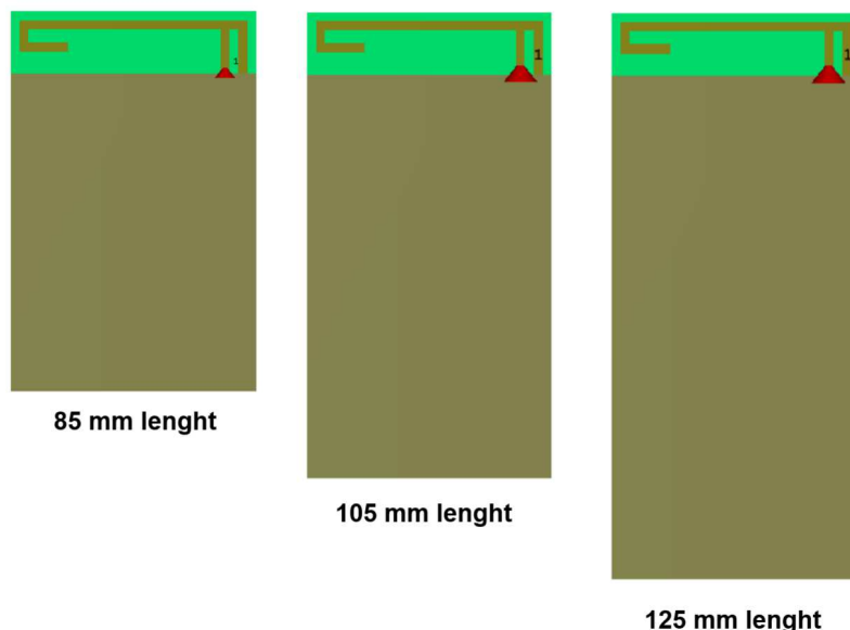
48 F antenna with change in length of PCB (A8)
