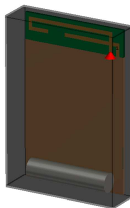
Dual IFA with battery V1
