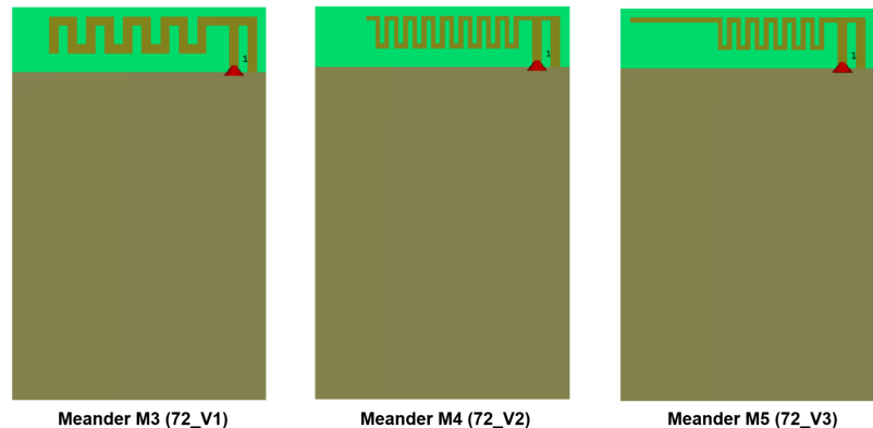
46 F antenna with change the meander (A72)
