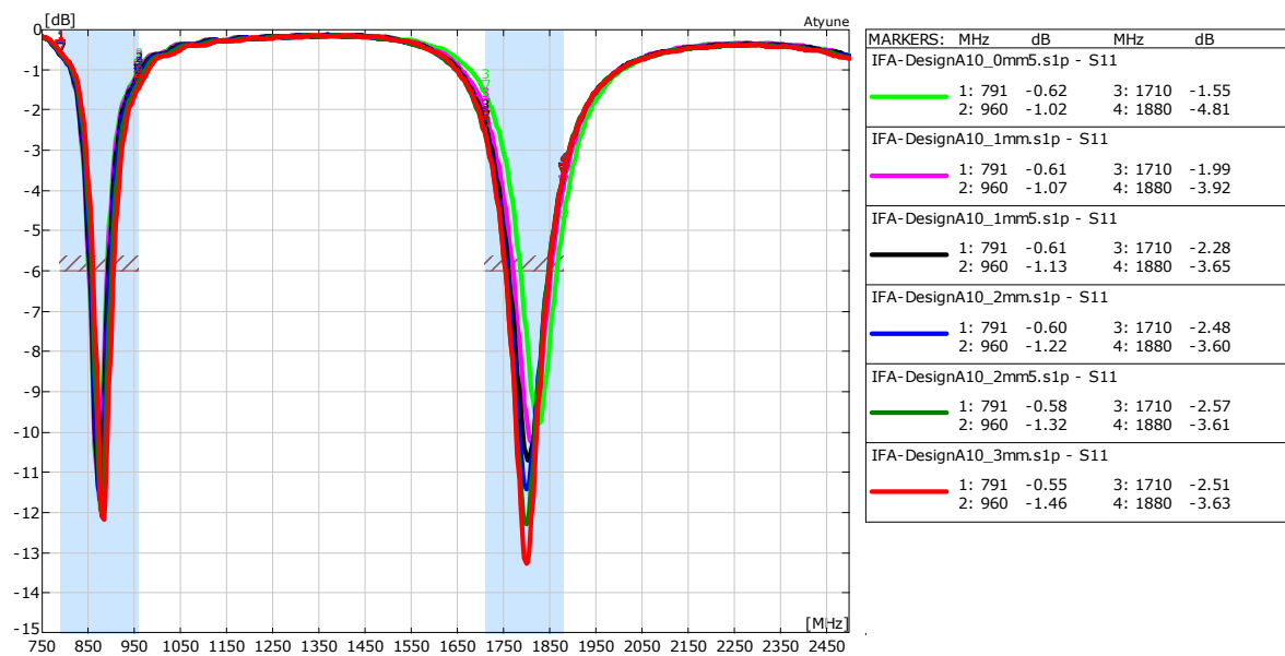
61 Dual F antenna of the width of the radiator (A10)
