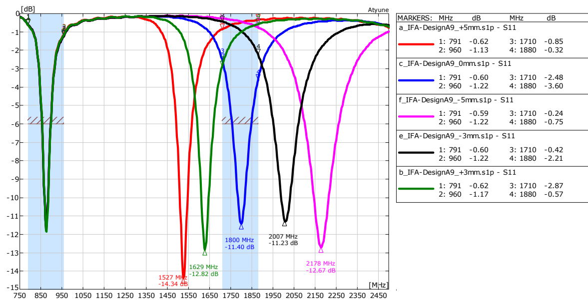
59 Return loss Dual F antenna with change in length of radiator (A9)
