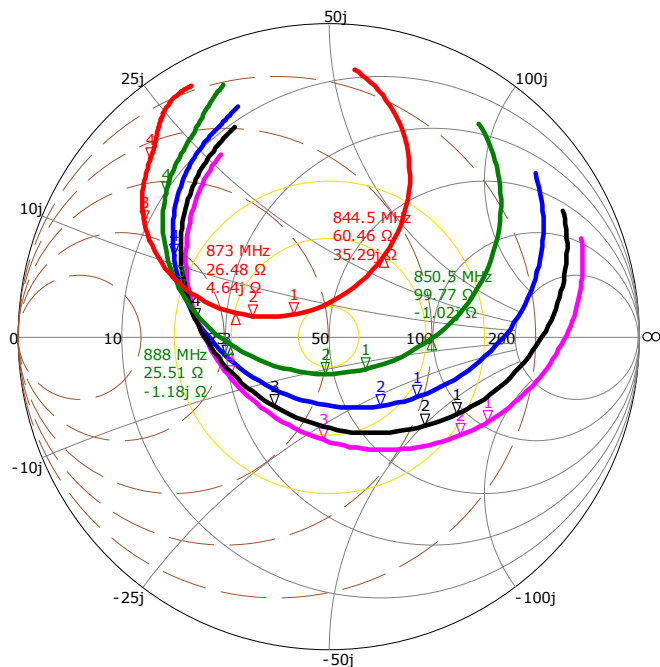
36 Smith Chart of F-antenna with change of distance to short-circuit point (A4withA8)
