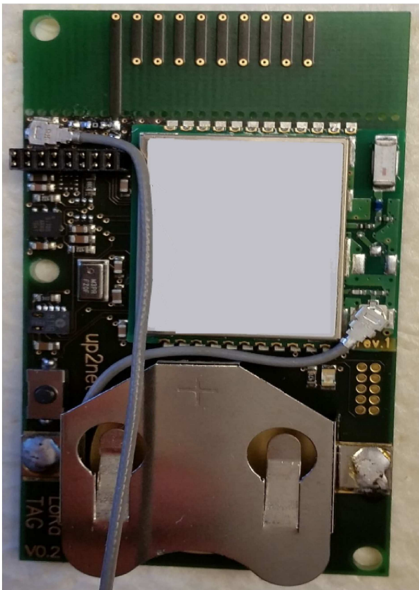
79 LoRa tag without enclosure
