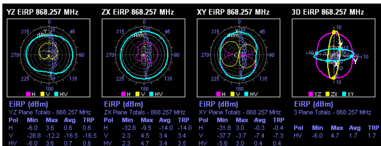
75 Radiated energy in 3 axes measured with MegiQ RMS
