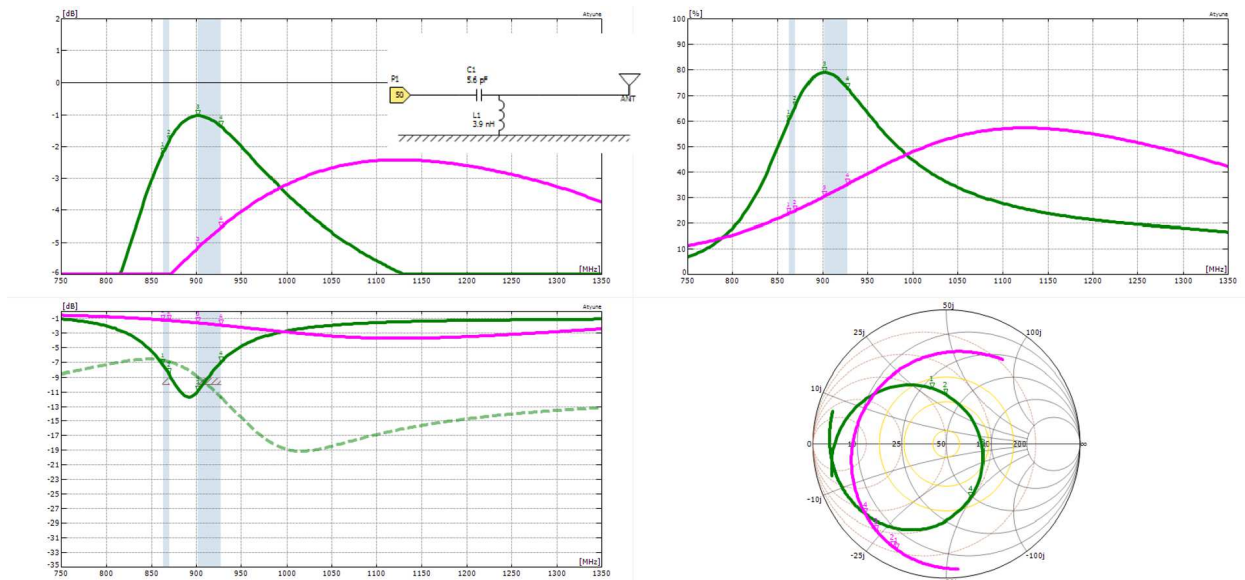
20 Gain, efficiency, return loss and Smith Chart of the L-antenna (A1) with change of distance of radiator to ground plane, unmatched and matched version 2
