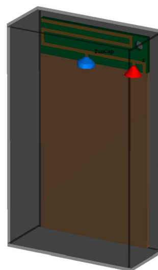
SIFA with tuning capacitor and enclosure
