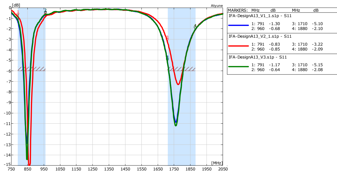
65 Return loss Dual F antenna with battery (A13)
