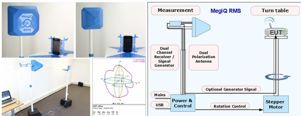
74 MegiQ RMS setup up to measure the radiated energy in 3 axes
