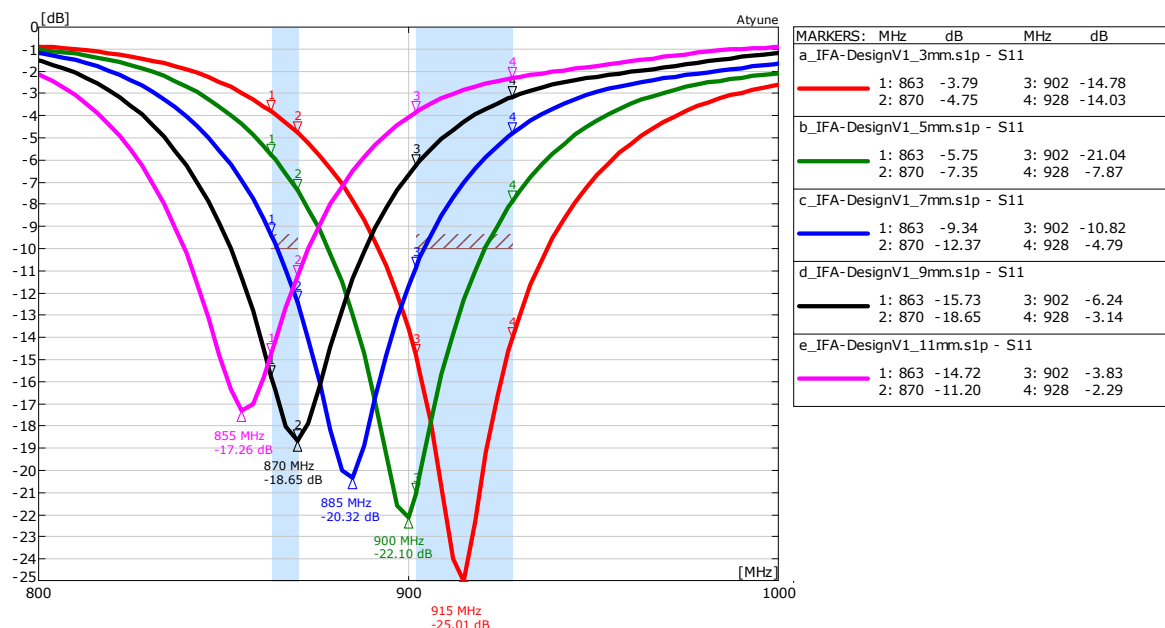
40 Return loss F antenna with change of radiator length (V1)
