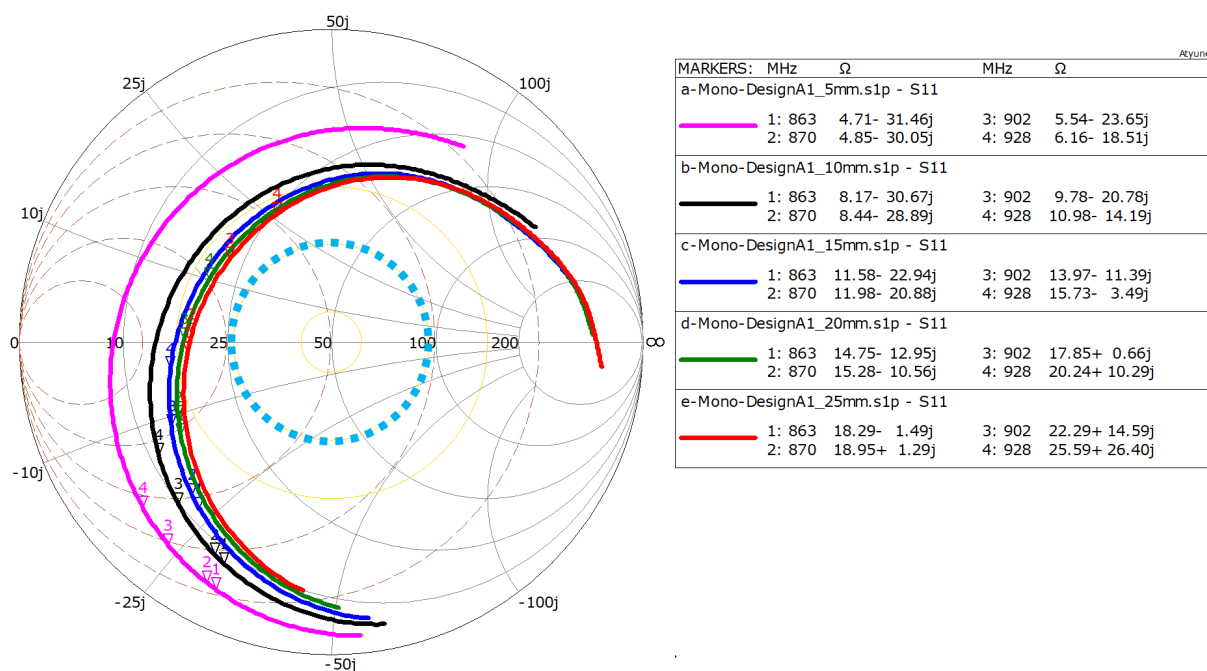
16 Smith Chart of L-antenna with change of distance of radiator to ground plane (A1)
