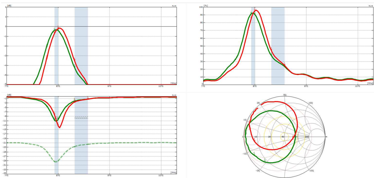
70 Gain, efficiency, return loss and Smith Chart for antenna V
