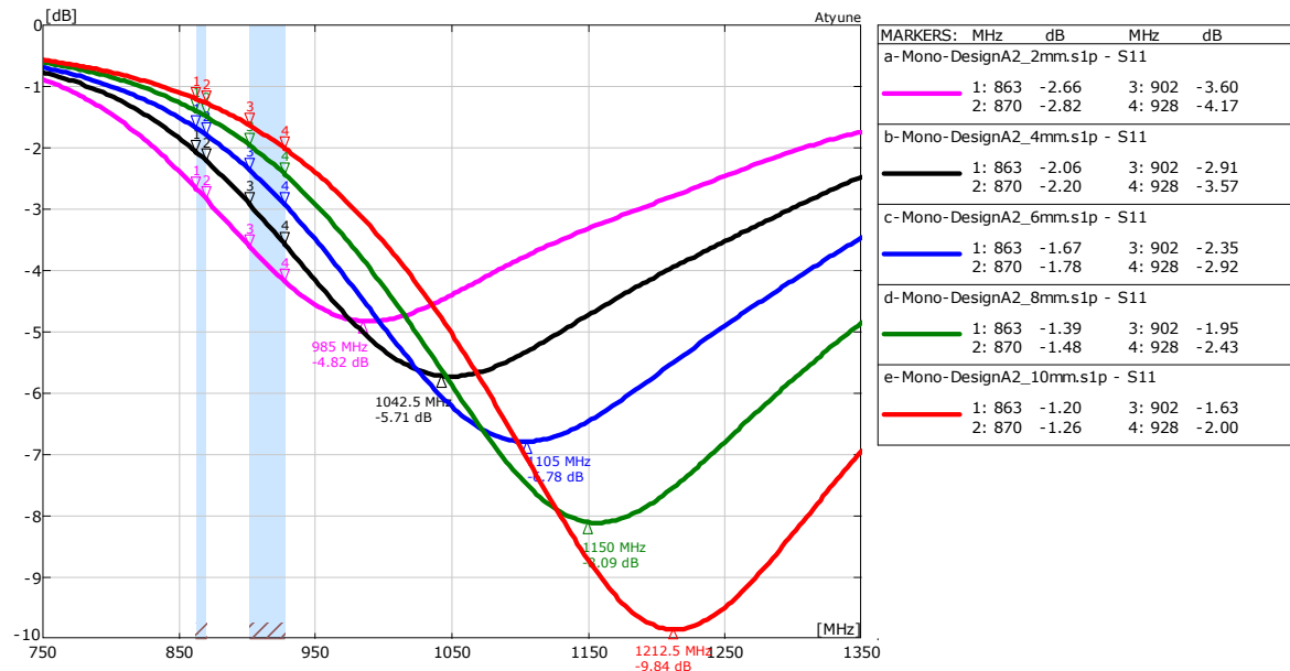
22 Return loss of the L-antenna with change of trace width at feed point
