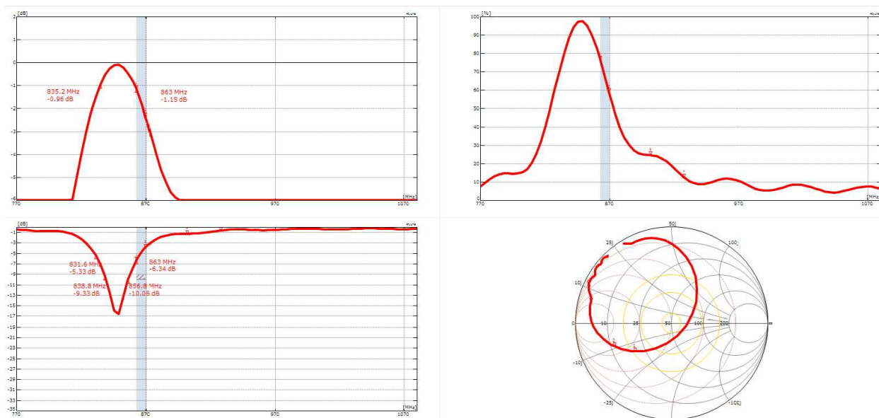
73 Gain, efficiency, return loss and Smith Chart for antenna inside the plastic enclosure at 850 MHz
