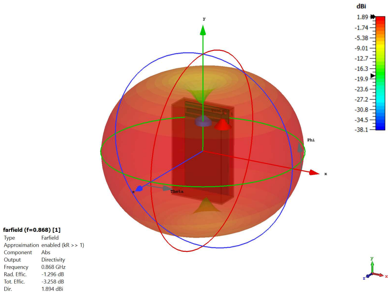
76 Simulation of the radiated energy in 3D at 868 MHz
