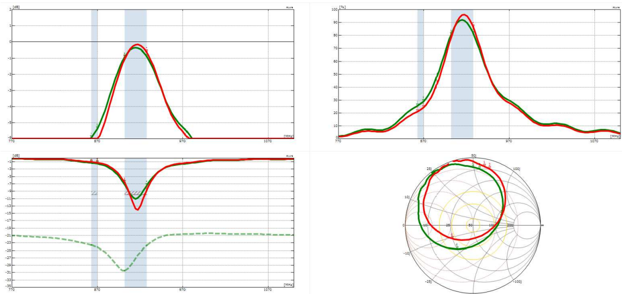
67 Gain, efficiency, return loss and Smith Chart for antenna II
