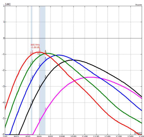
15 Gain in dB and efficiency of L-antenna with change of distance of radiator to ground plane (A1)
