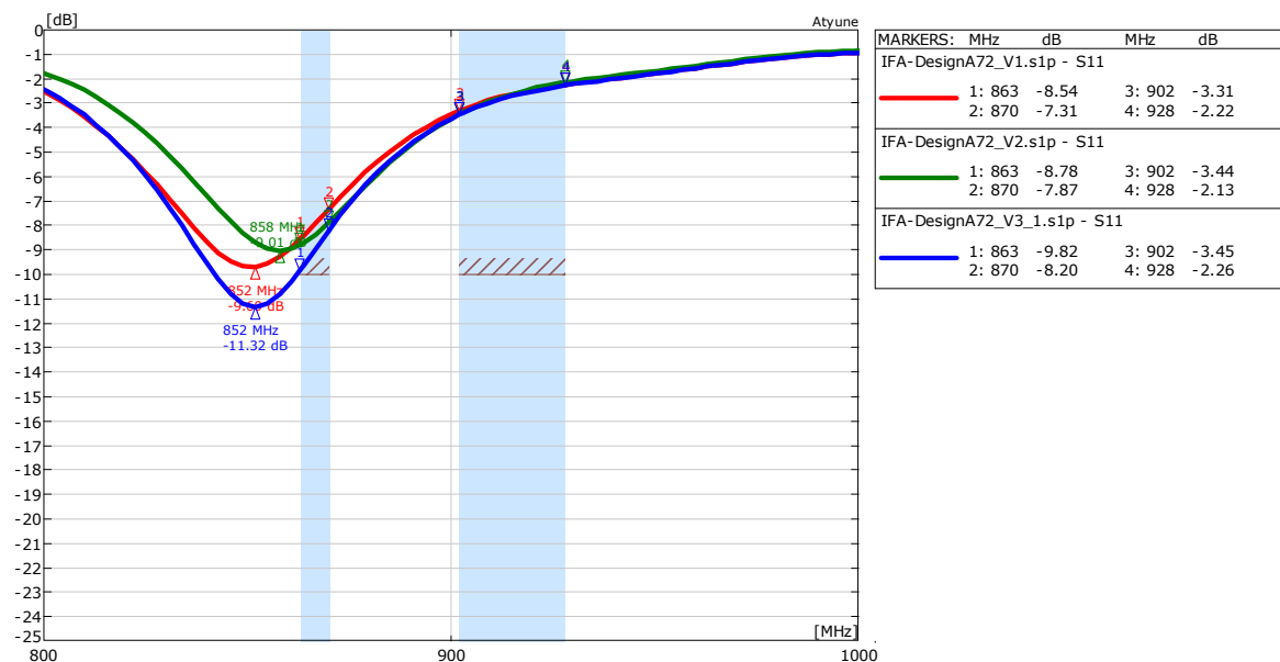
47 F antenna with change of PCB length (A72)
