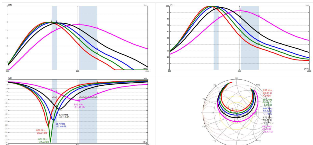
29 Gain, efficiency, return loss and Smith Chart of F antenna with change of trace width at feed point (A2withA8)
