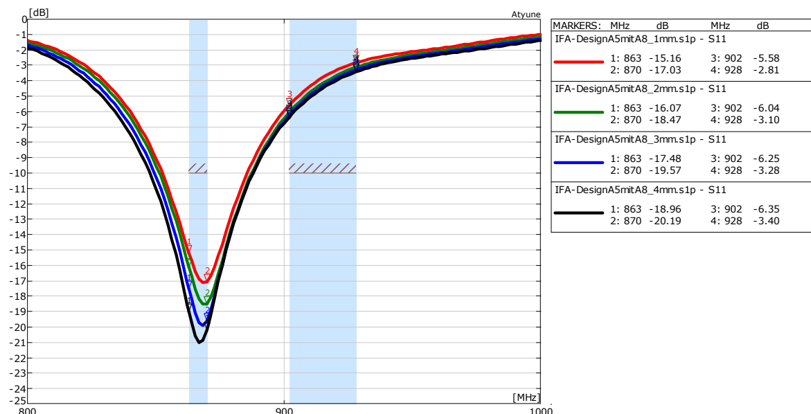
37 F antenna with change of radiator width (A5withA8)
