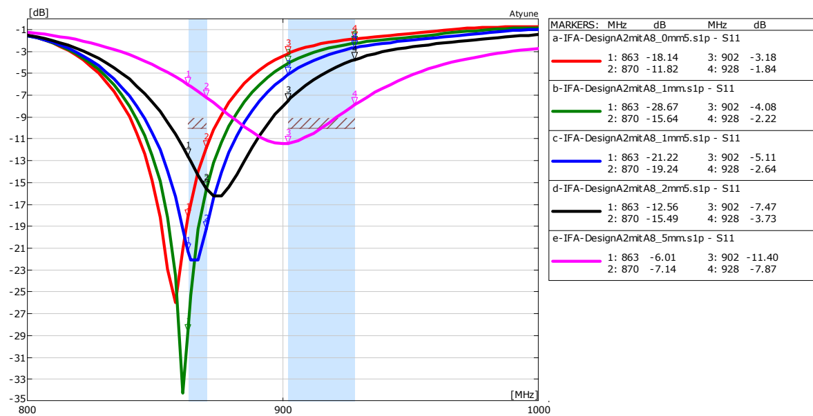
28 Return loss F antenna with change of trace width at feed point (A2withA8)
