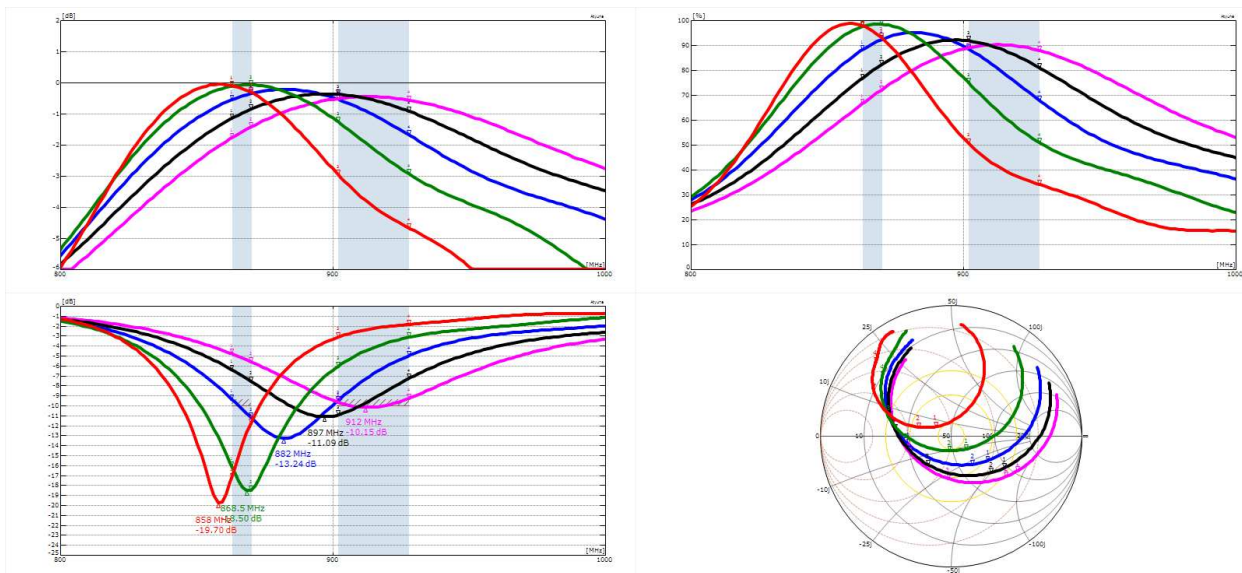
35 Gain, efficiency, return loss and Smith Chart of F-antenna with change of distance to short-circuit point (A4withA8)
