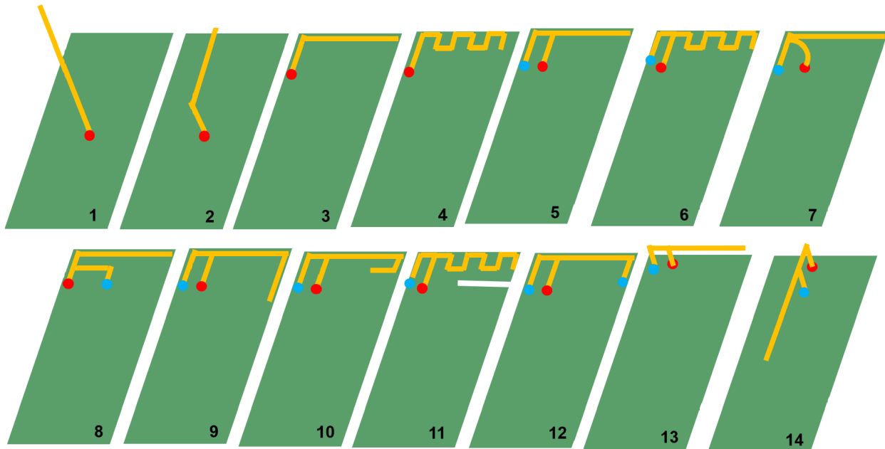
7 Overview of different L- and F antennas
