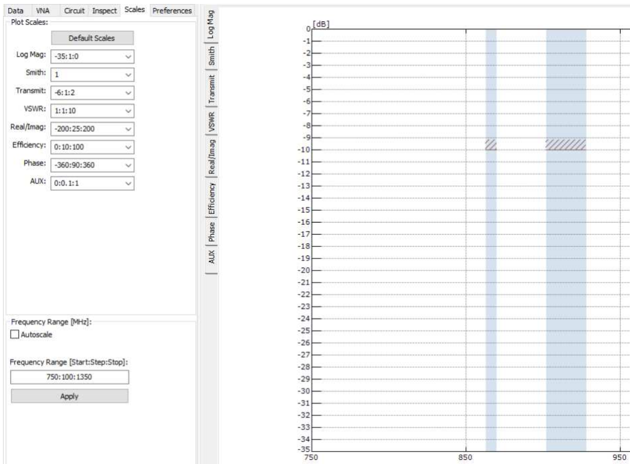
11 Setup of the scales at software Atyune
