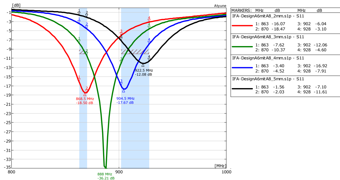
42 Return loss of F-antenna with change of the width of the short-circuit point (A6withA8)
