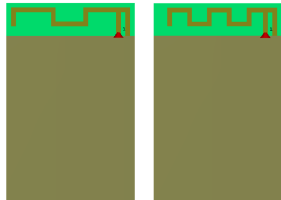
Meander M1 (A70_1) Meander M2 (A71) 43 F antenna with meander (A70&A71)
