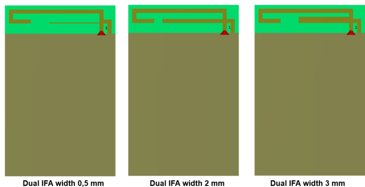
60 Dual F antenna of the width of the radiator (A10)
