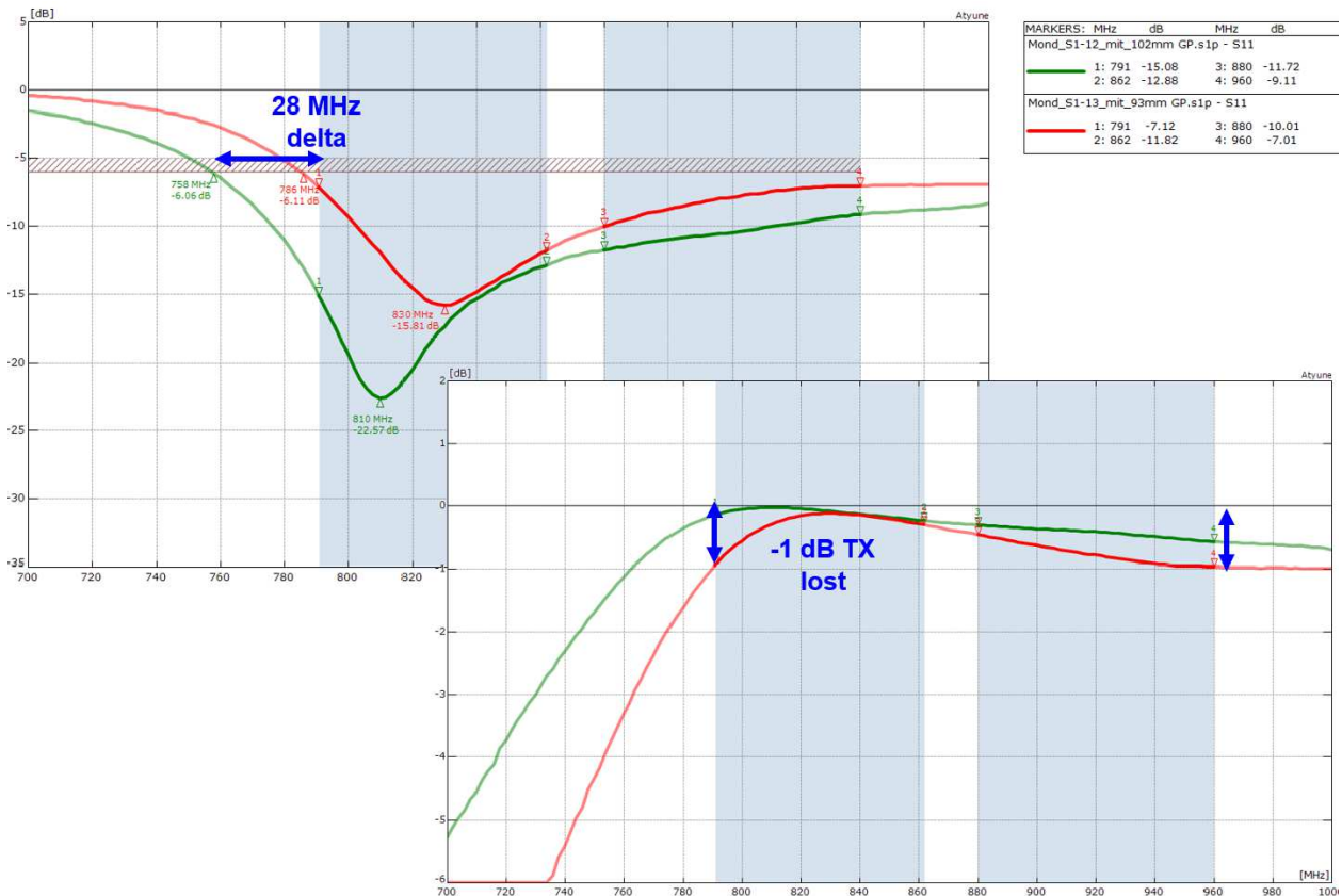
91 Return loss of NB-IoT chip antenna on 93 mm and 102 mm long ground plane
