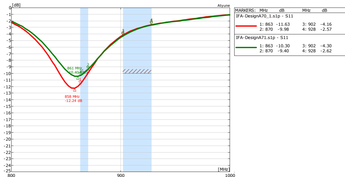
44 Return loss F antenna with meander (A70&A71)
