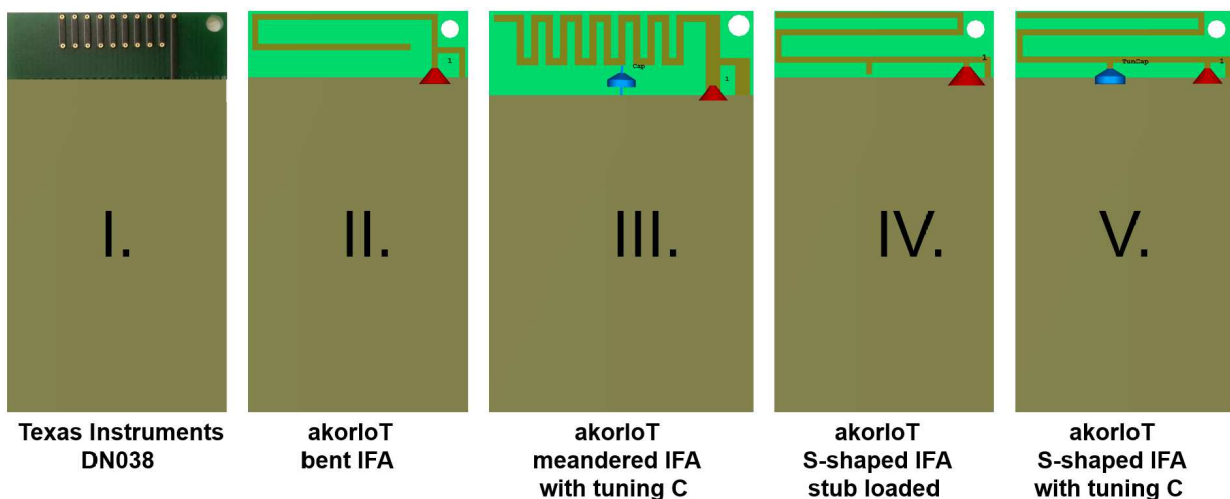
66 Antenna I based on TI DN038. Antenna II to V on same PCB space but better performance
