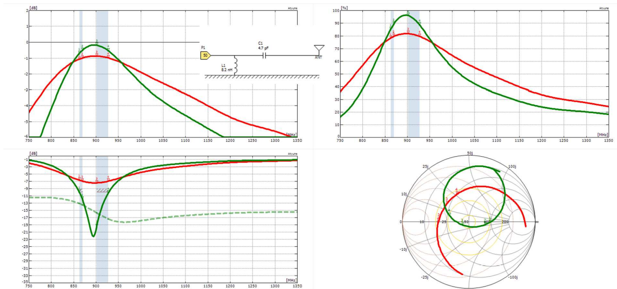
19 Gain, efficiency, return loss and Smith Chart of the L-antenna (A1) with change of distance of radiator to ground plane, unmatched and matched version 1
